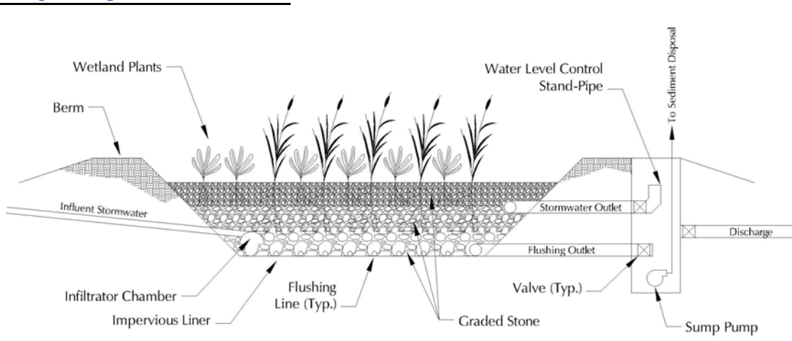
Schematic of stormwater treatment wetland.
